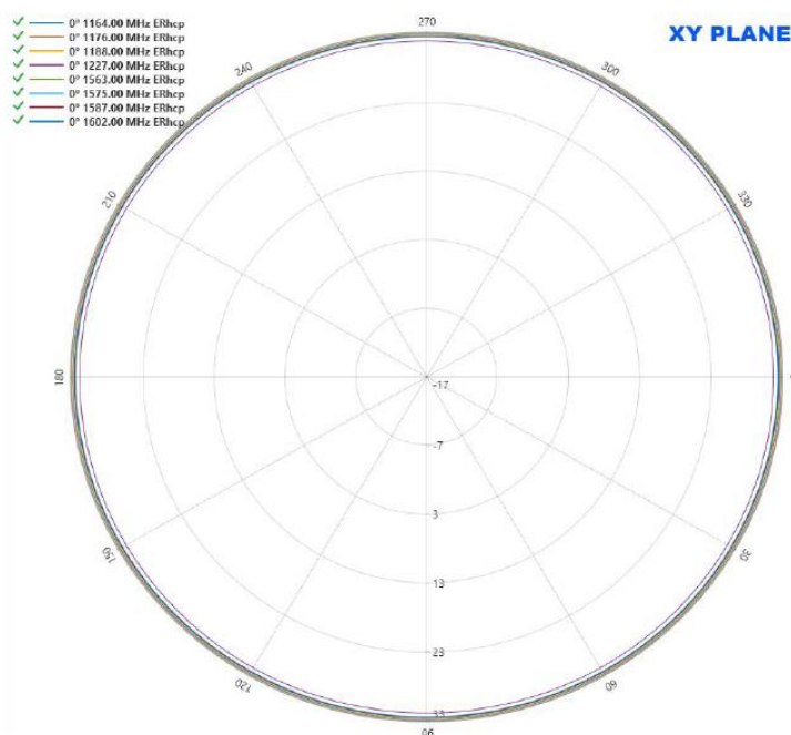
GNSS Antenna
